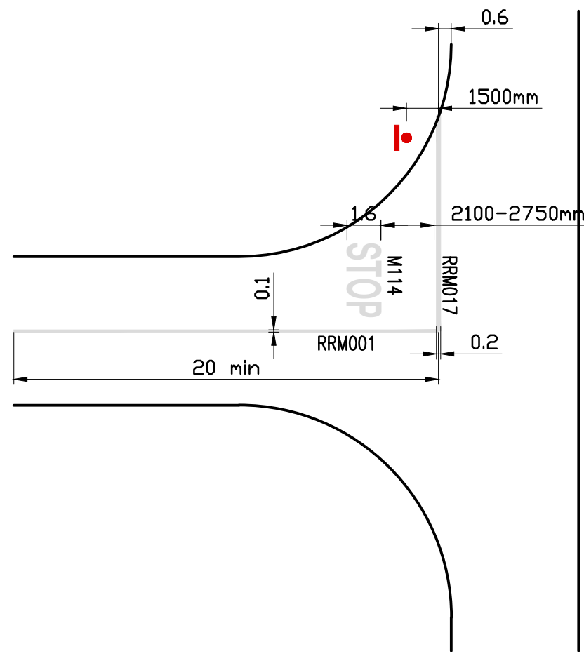
PRIORITY CONTROLLED STOP JUNCTION SCALE 1:250
