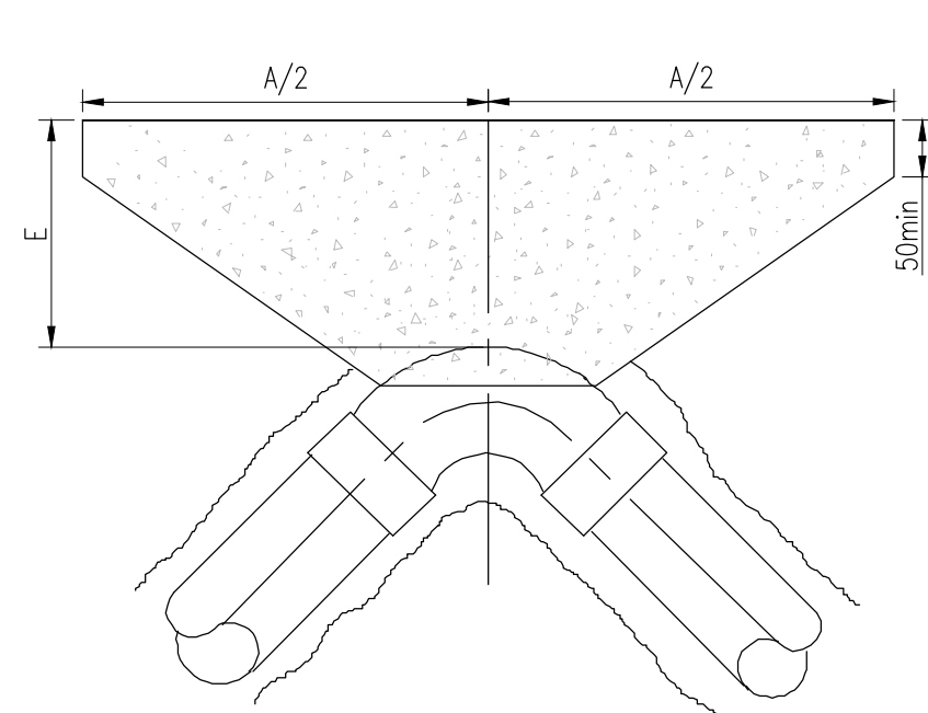
90 DEGREE BEND
