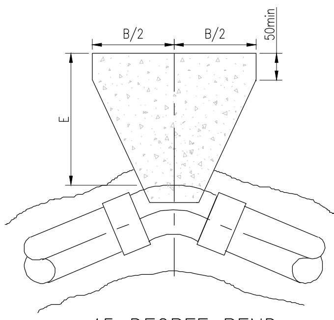
45 DEGREE BEND
